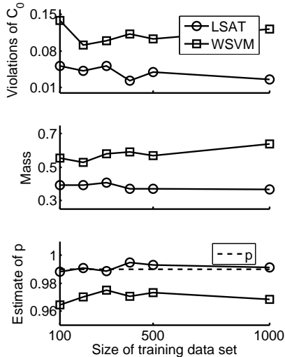
Fig. 1. Synthetic data set. Fraction of included points violating C_0 (TOP), mass (MIDDLE) and probability of avoiding small return (BOTTOM) of G as a function of number of points used for training. Testing was performed using 2000 data points.
